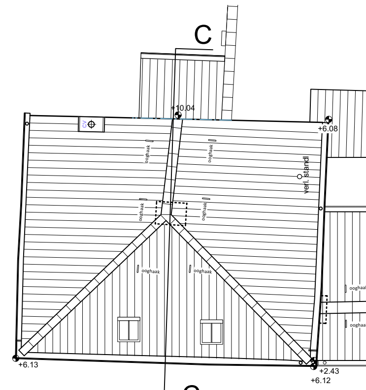
DAKENPLAN
